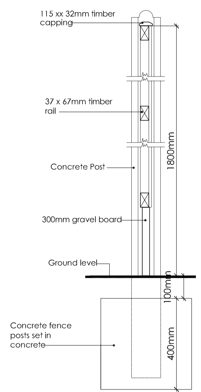
Section 1:10 Fence Type A
