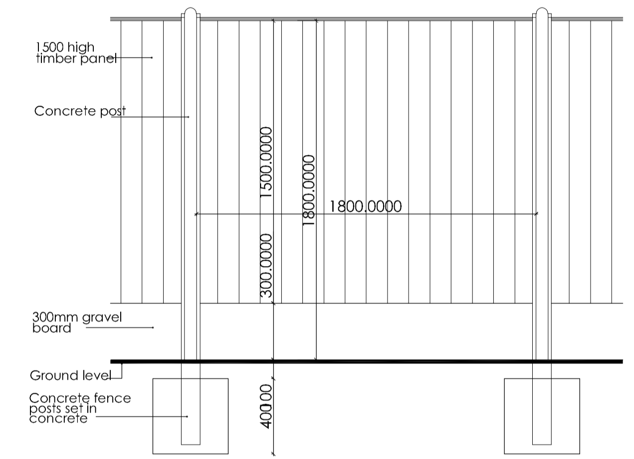
Elevation Fence Type A 1:20
